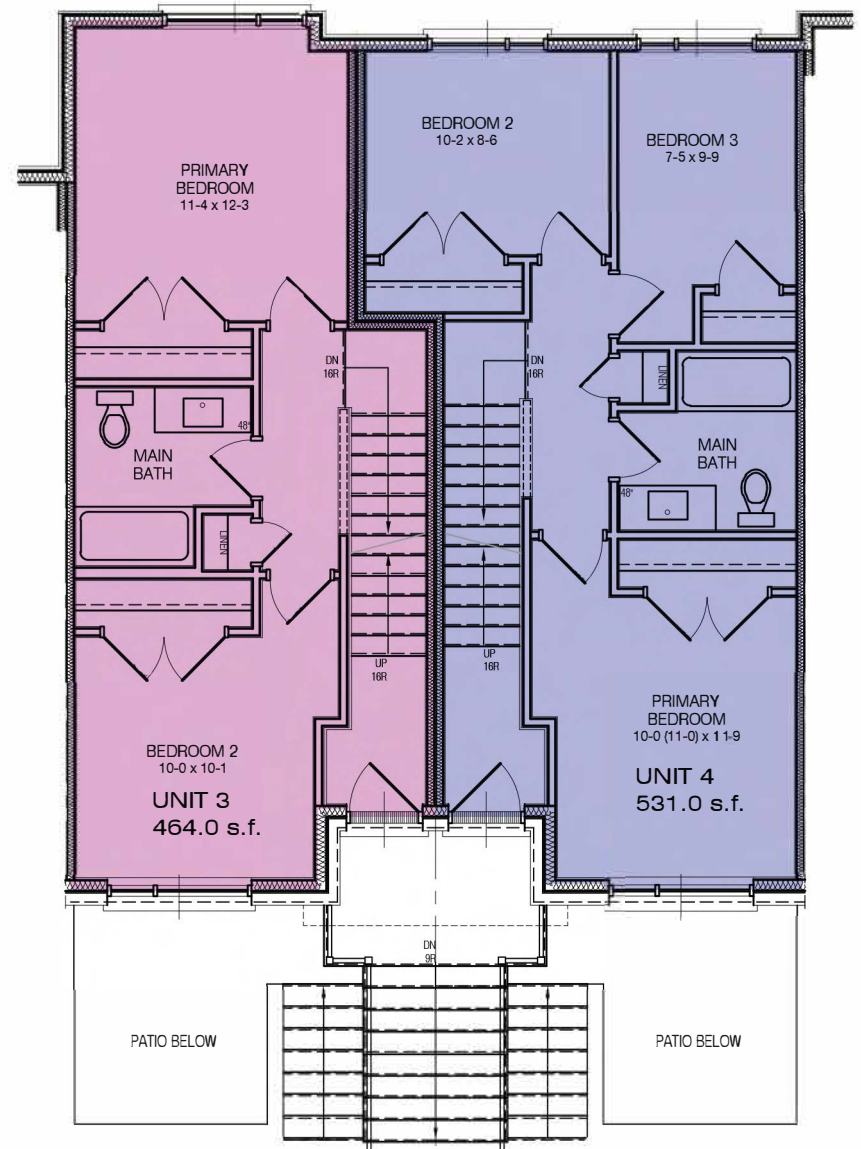
LEVEL 2 FLOOR PLAN
