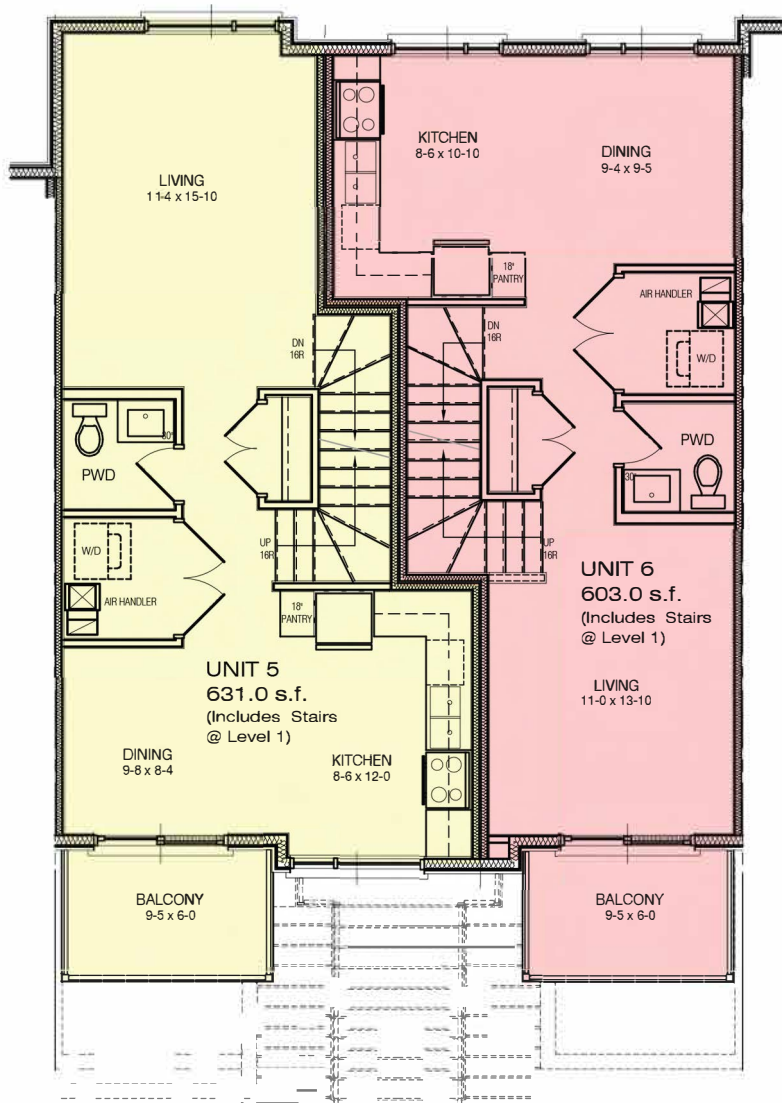
LEVEL 3 FLOOR PLAN
